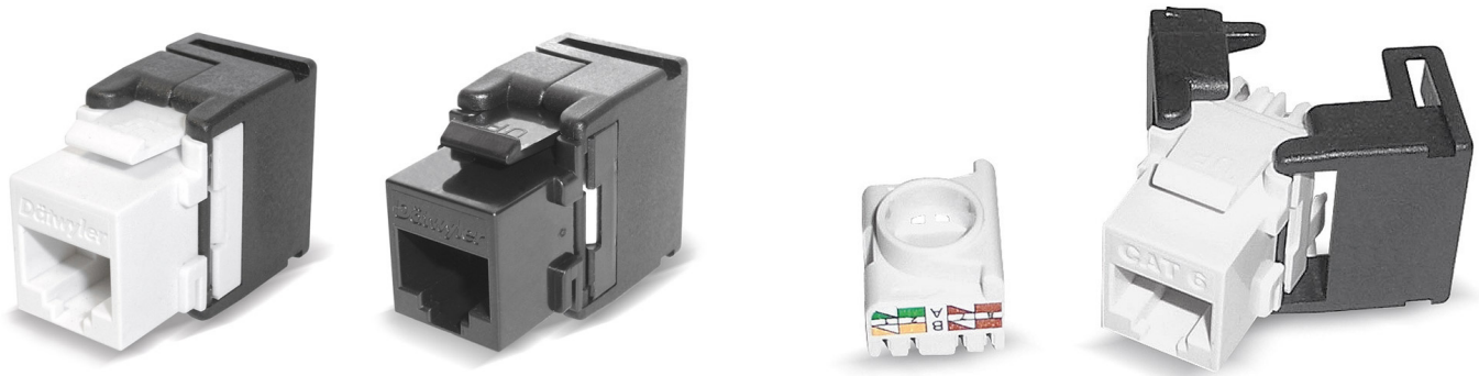
KU-T 1/8 tool-less RJ45 module, unshielded, Cat.5e, in white or black
