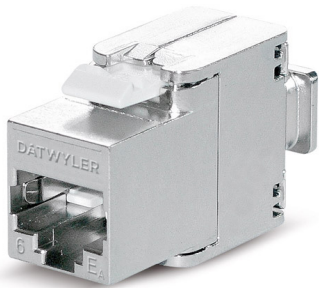
KS-TS 1/8 tool-less slimline Cat.6/EA RJ45 module
