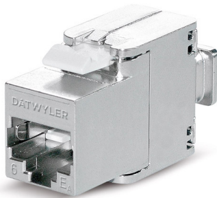
RJ45 module KS-TS 1/8 tool-less slimline Cat.6/EA
