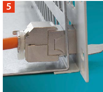
5 Modul in finaler Position Jack in final position
